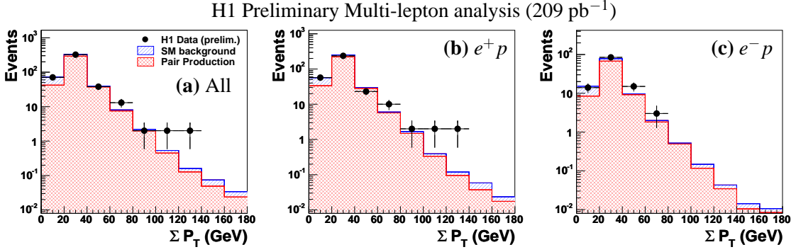
Figure 1: Distributions of the scalar sum of the transverse momenta of leptons compared to expectations for all data (a) and separately for events recorded in e^+p (b) and e^-p (c) collisions.
