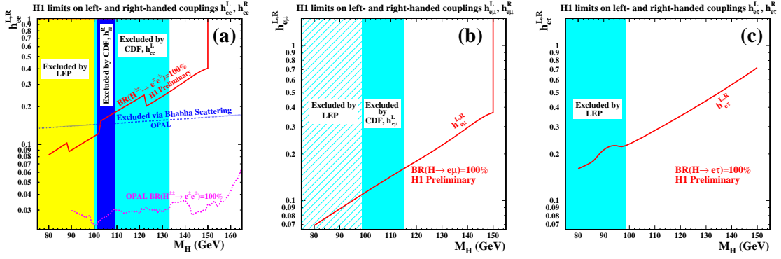
Figure 2: Upper limits at 95% confidence level on the coupling h_{ee} as a function of the doubly-charged Higgs mass assuming that the H^{\pm\pm} only couples to electrons (a). Regions above the curves are excluded. In (b) and (c) upper limits on the couplings h_{e\mu} and h_{e\tau} are shown, assuming that the H^{\pm\pm} only couples to e\mu and e\tau , respectively.
